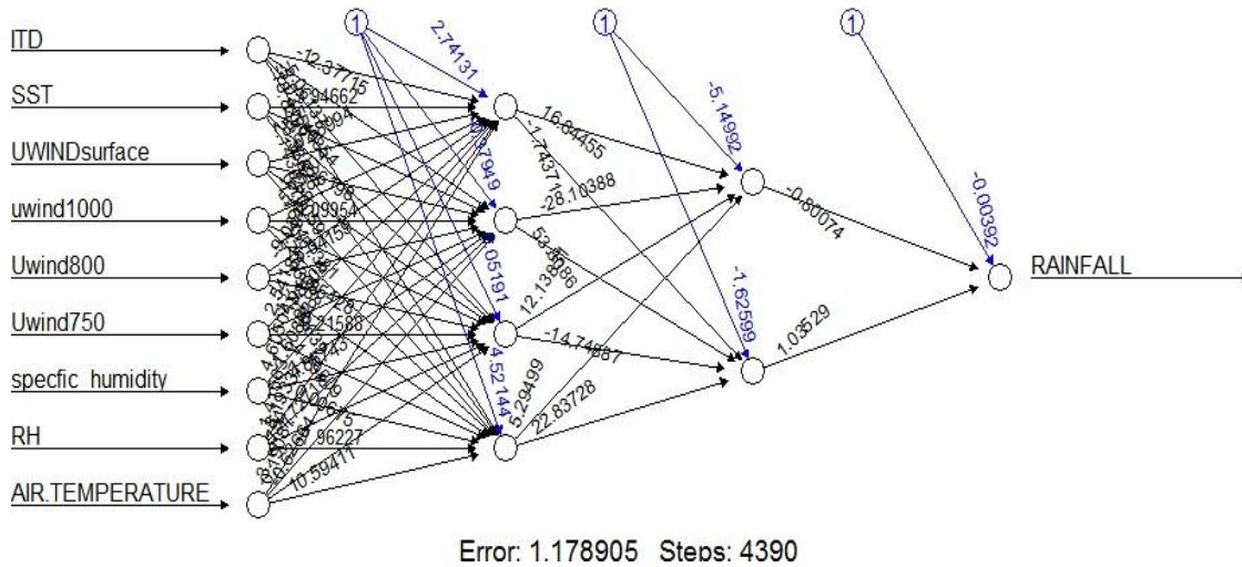
Fig. 1. ANN model architecture for the nine input (9) parameters, 4 hidden layers and the final output (rainfall) parameter
