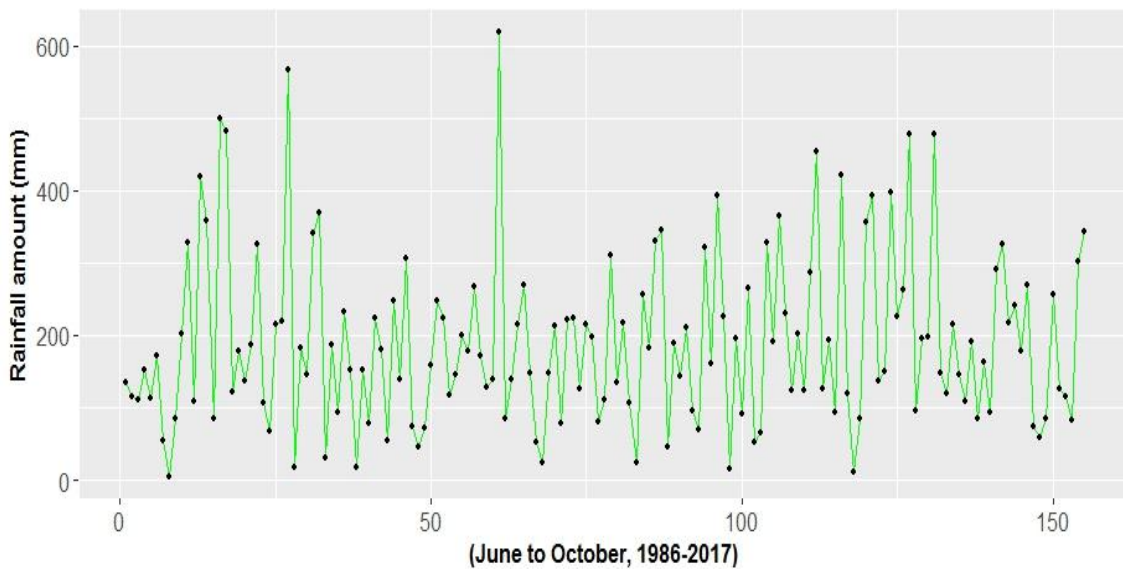
Fig. 2. Seasonal rainfall amount for the period of June to October from 1986 to 2017 in Ikeja
