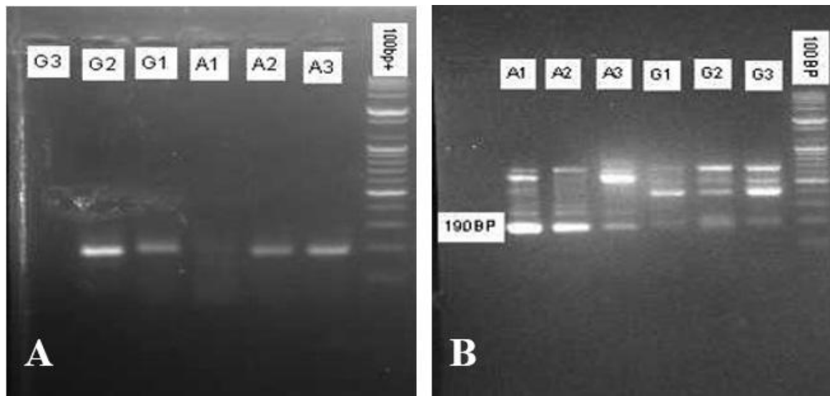
Fig. 5. PCR band for 12SrRNA gene amplification of the Simulium spp. (196bp), lane G1-G3 and A1-A3 are Simulium spp(A) and PCR band for 0-150OVgene amplification of Onchocerca volvulus from the Simulium spp. (190bp), G1-G3 and A1-A3 are O. volvulus DNA from Simulium spp. (B)
