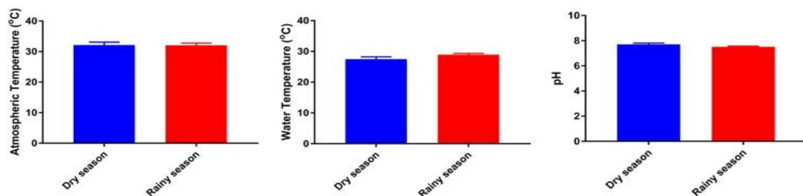
Fig. 2. The pH, atmospheric and water temperatures at Gamji park Kaduna. Values are presented as mean ± SEM, * indicates significant difference at P < 0.05, SEM = standard error of mean
