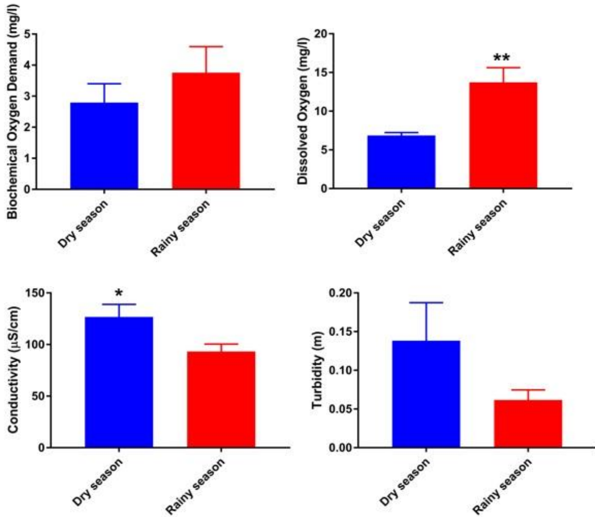
Fig. 3. Biochemical oxygen demand, dissolved oxygen, conductivity and turbidity at Gamji park Kaduna. Values are presented as mean \pm SEM, ** indicates significant difference at P<0.05, SEM= standard error of mean
