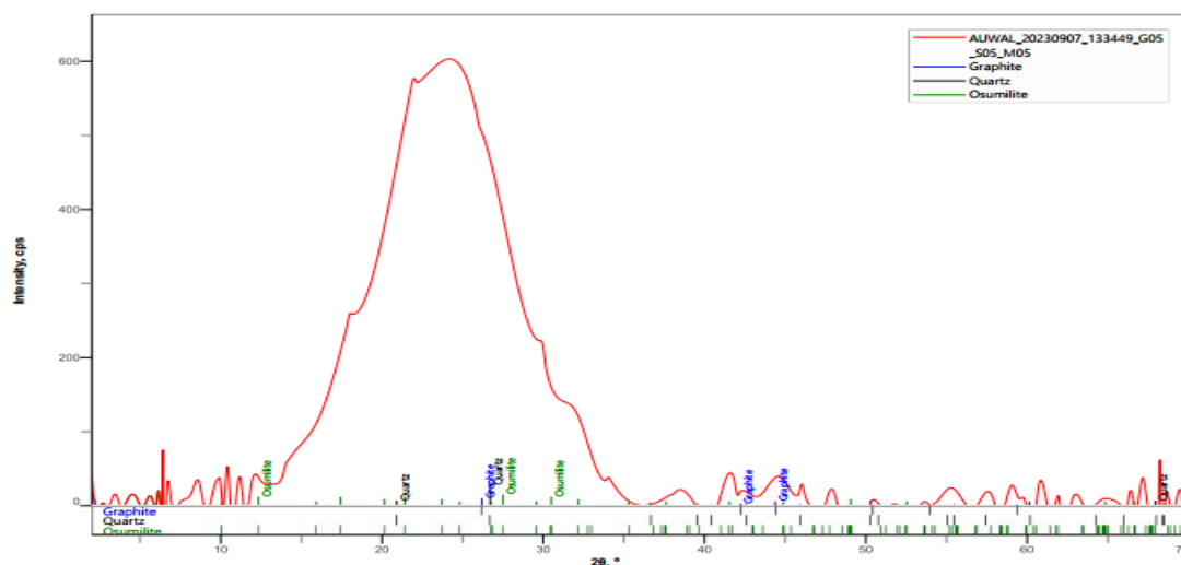
Fig. 5. XRD Analysis of the unimpregnated MHFS
