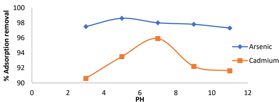
Fig. 9. Effect of pH
