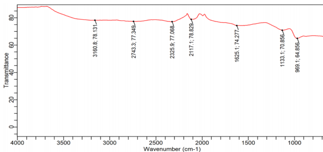
Fig. 1. FTIR Analysis of the unimpregnated MHFS
