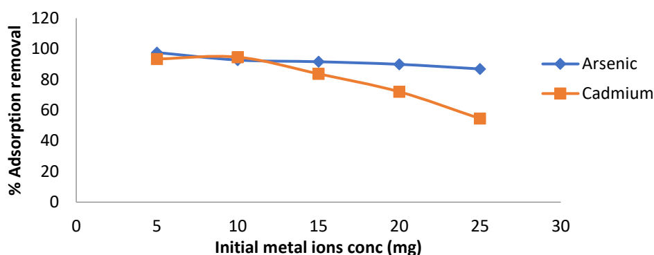
Fig. 7. Effect of initial concentration
