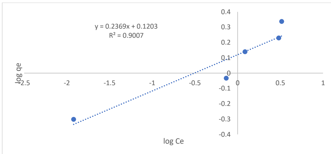
Fig. 13. Freundlich for as on MHFS
