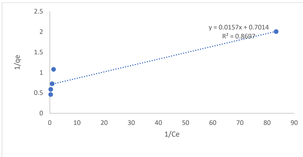
Fig. 12. Langmuir for as on MHFS
