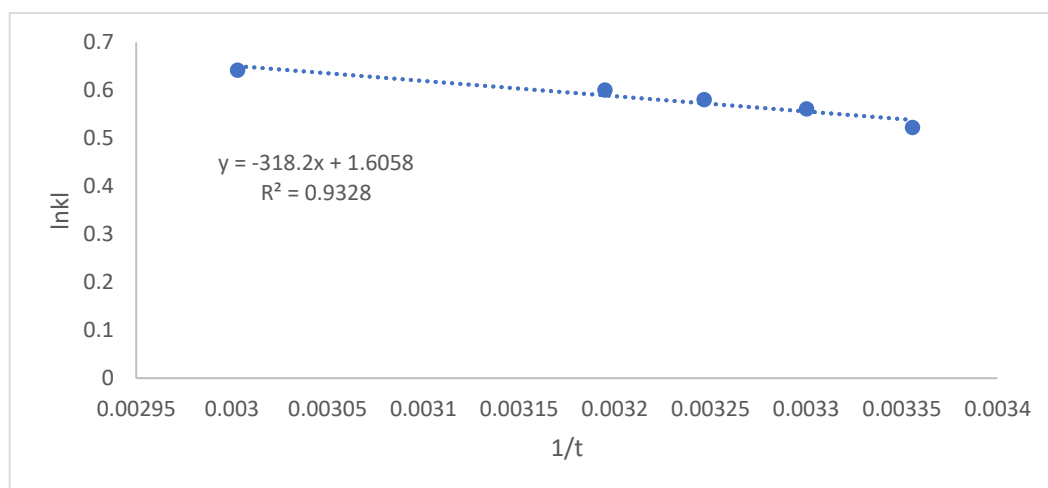
Fig. 21. Thermodynamic on Cd for MHFS
