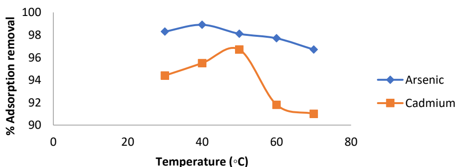
Fig. 10. Effect of temperature
