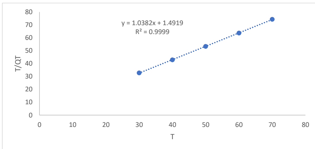
Fig. 19. Pseudo second order for Cd on MHFS
