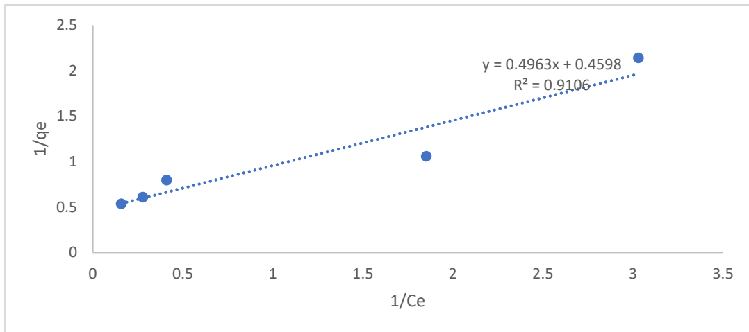
Fig. 14. Langmuir for Cd on MHFS
