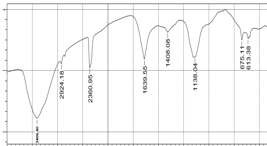
Fig. 2. FTIR analysis of the impregnated MHFS SEM Analysis of the Adsorbent
