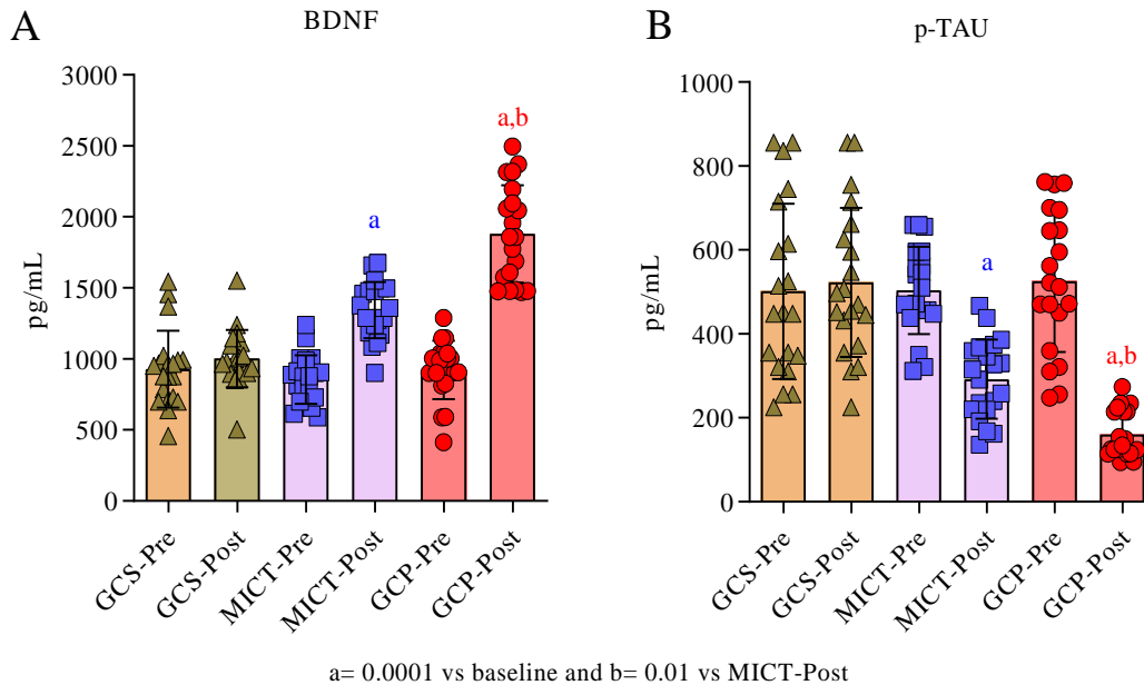
Fig. 2. BDNF and p-TAU quantification
