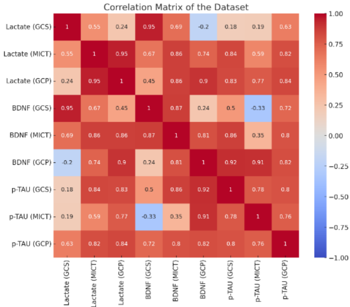
Fig. 3. Correlation matrix
