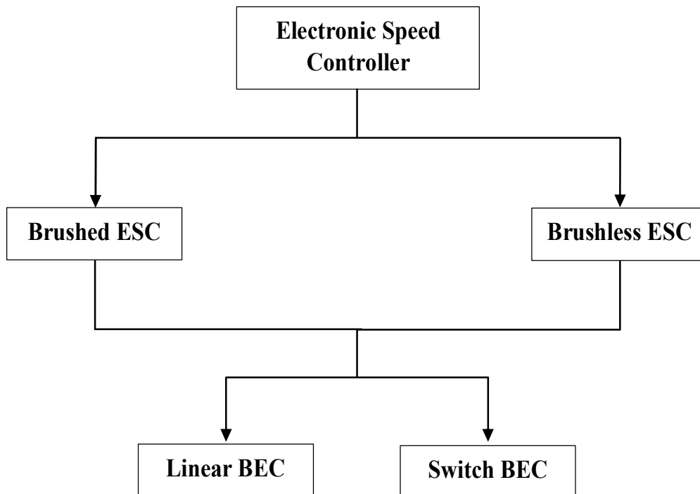
Fig. 16. Classification of ESC
