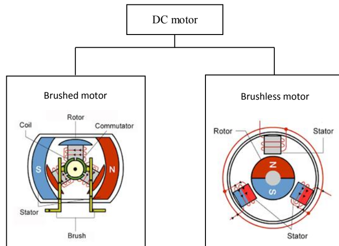
Fig. 12. Classification of DC motor
