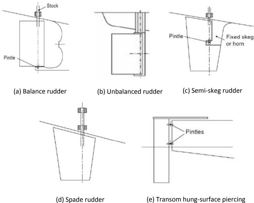
Fig. 13. Different types of rudder in a conventional propeller-rudder systems [44]
