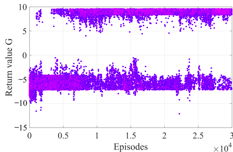
Figure 10. The return value of the DDPG during training.
