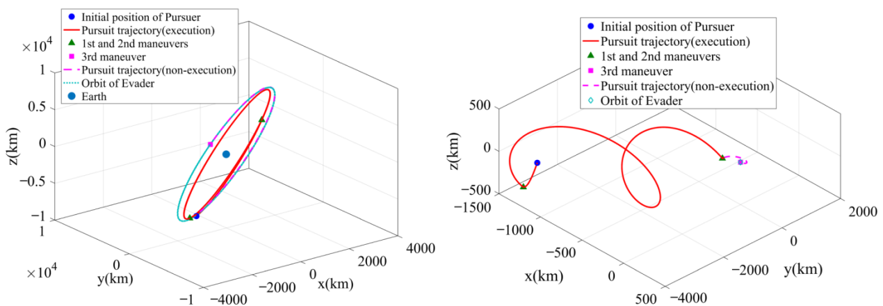
Figure 7. The pursuit trajectory of the FRS for case A ( left is the pursuit trajectory in J2000 Earth-centered inertial frame; right is the pursuit trajectory in the orbital coordinate system of the evader).
