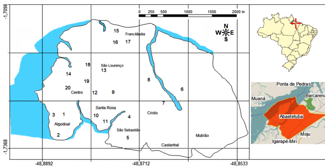
Fig. 1. Location of the municipality of Abaetetuba (Pará, Brazil) with indication of monitored tubular wells
