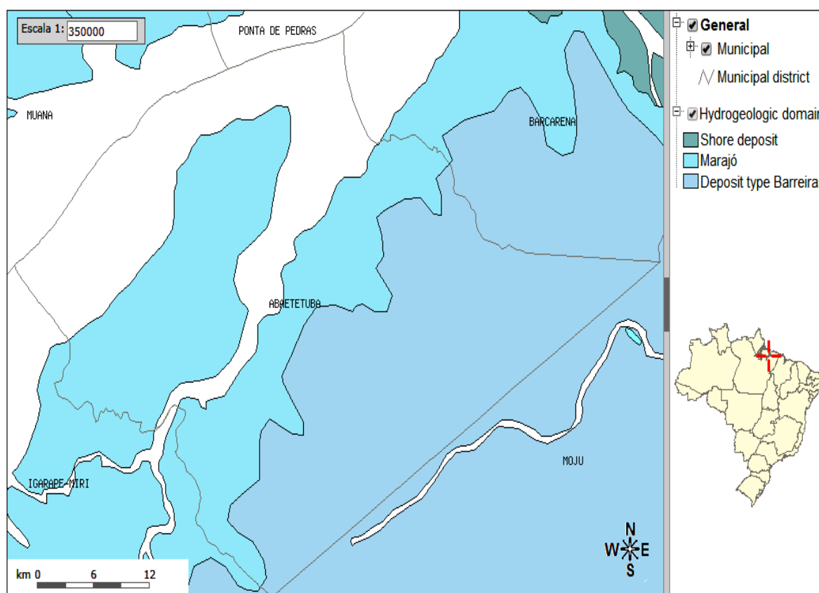
Fig. 3. Hydrogeological domains observed in the limits of the municipality of Abaetetuba (Pará, Brazil)
