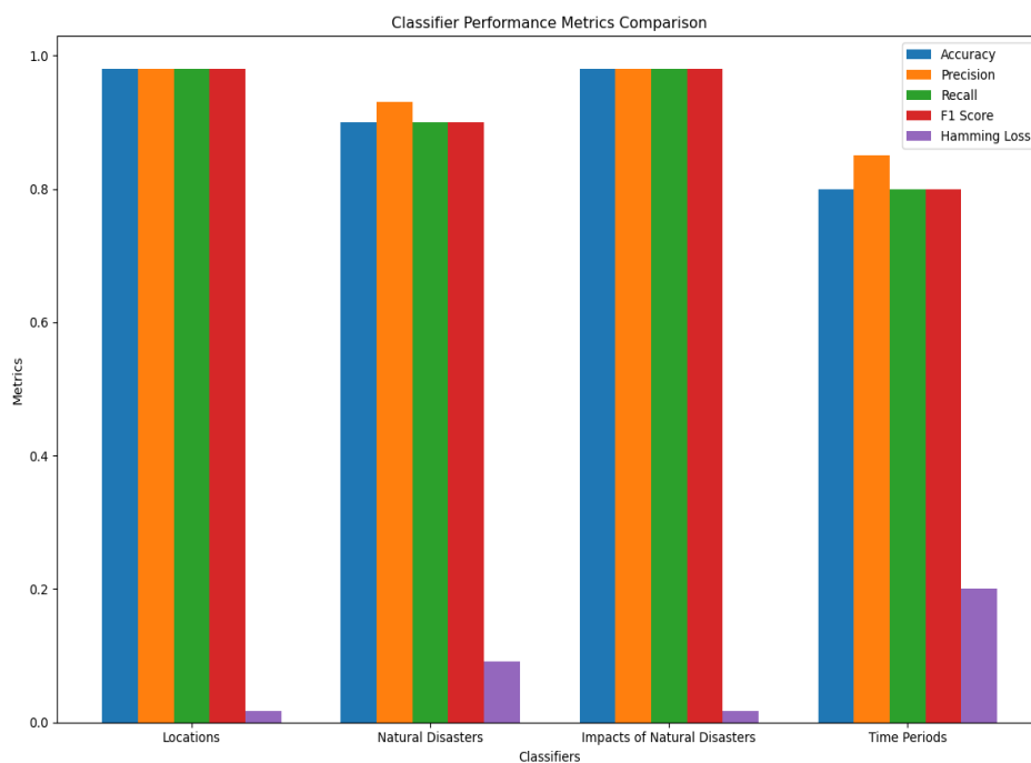
Fig. 2. Classifier performance comparison chart
